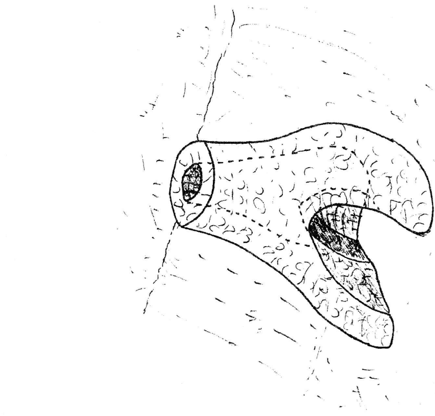
Figure 2. A typical horseshoe kiln. If possible this would be built against a slope so that it could easily be loaded from the top whilst still allowing access to the drawhole for unloading.
